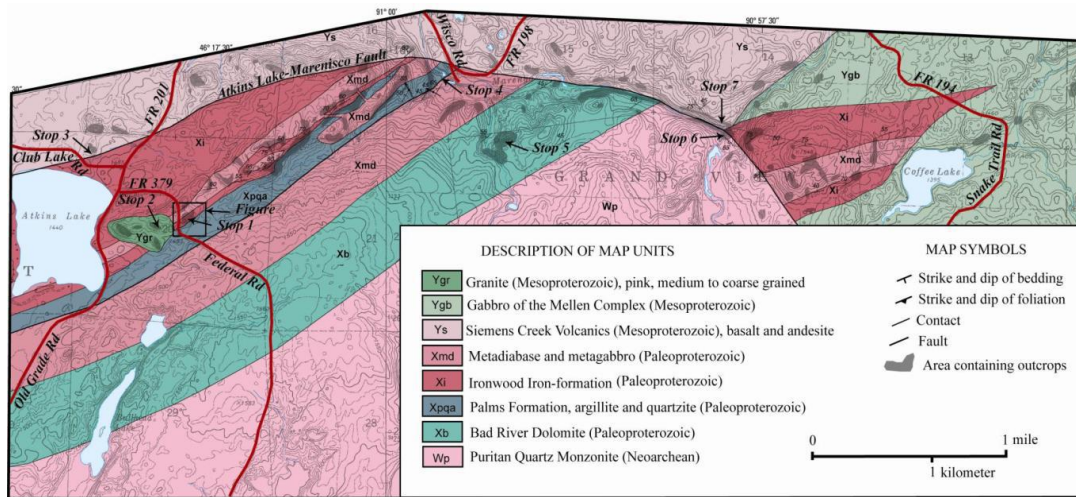
Figure 1. Geologic map of the Atkins Lake-Marengo Falls area showing the location of field trip stops. Geology from Cannon et al. (1996)
